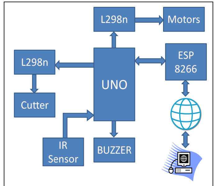
Fig. 1. Block diagram of Lawn Mower.
