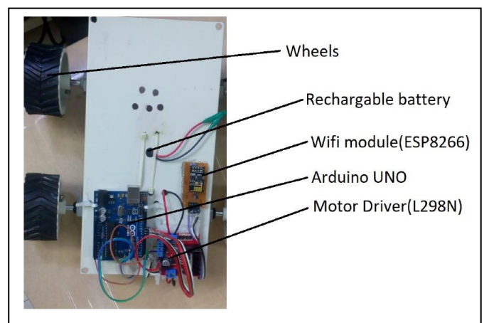
Fig. 3. Circuitry of Lawn Mower
