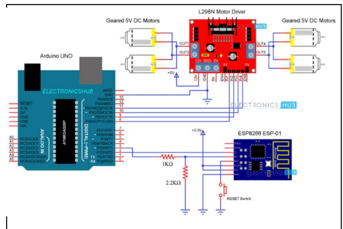
Fig. 2. Circuit diagram of Lawn Mower.
